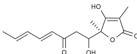
Fig. 4: Antimicrobial butenolide structures: Trichoderma longibrachiatum (5-hydroxyvertinolide)
