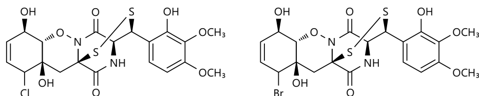
Fig. 2: Structures of gliovirin analogues derived from Trichoderma longibrachiatum diketopiperazines
