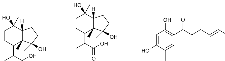
Fig. 6: 10,11-dihydrocyclonerotriol, catenioblin C and sohirnone A
