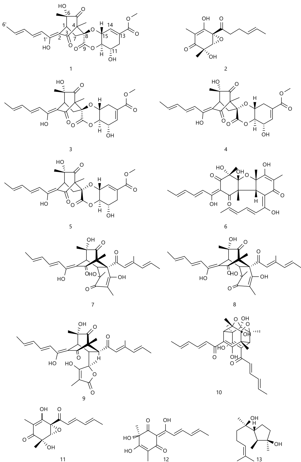
Fig. 5: Chemical compositions of compounds 1 to 13 discovered in Trichoderma longibrachiatum SFC100166
